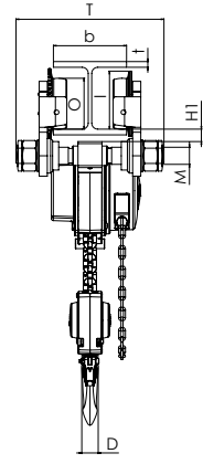
PLAIN TROLLEY HOIST 5 TON
