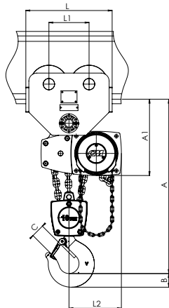
GEARED TROLLEY HOIST 10 TON
