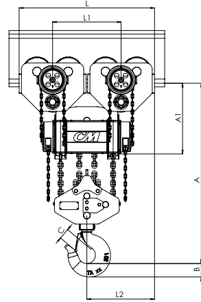
GEARED TROLLEY HOIST 15 & 20 TON
